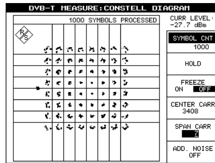
Fig. 7 Constellation diagram with corrected Q component offset. I component offset not yet optimized (conchoids of I/Q value pairs open to the inside).
