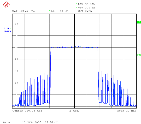
Fig.10 Impulsive Noise and DVB-T spectrum with BER = 2 \cdot 10^{-4} after Viterbi.
