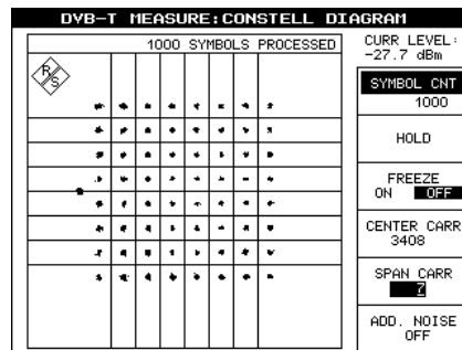
Fig. 8 Optimally aligned constellation diagram in 8k mode with residual carrier suppression >25 \text{ dB} .
