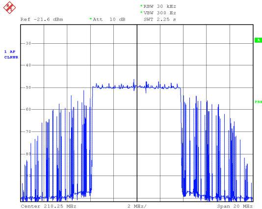
Fig. 13 Noise floor at 50 dB of DVB-T spectrum with superposed impulsive noise (max.power) at 50 dB
