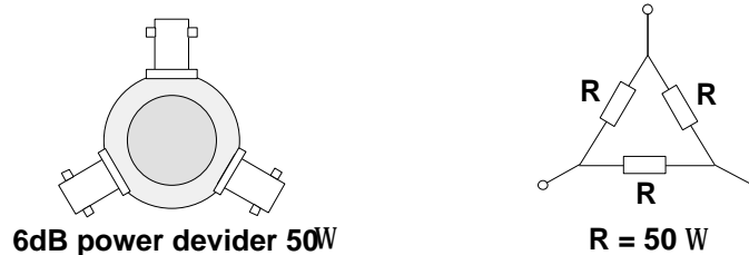
Fig. 2 50 Ω, 6 dB power divider; mechanical design and schematic diagram
