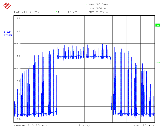
Fig. 15 Noise floor at 46 dB of DVB-T spectrum with superposed impulsive noise and extended dynamic range
