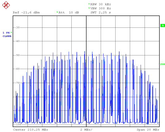
Fig. 12 Example: spectrum of impulsive noise at max. power
