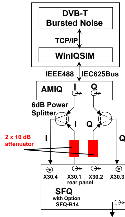
Fig. 14 Increasing the dynamic range of Impulsive Noise
