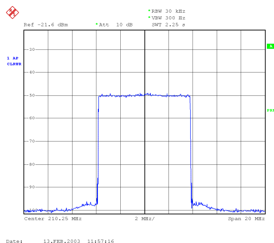
Fig. 11 Noise floor at 50 dB of test transmitter's DVB-T spectrum
