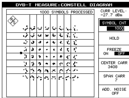
Fig. 6 Constellation diagram with corrected Q component offset. I component offset not yet optimized (conchoids of I/Q value pairs open to the outside).
